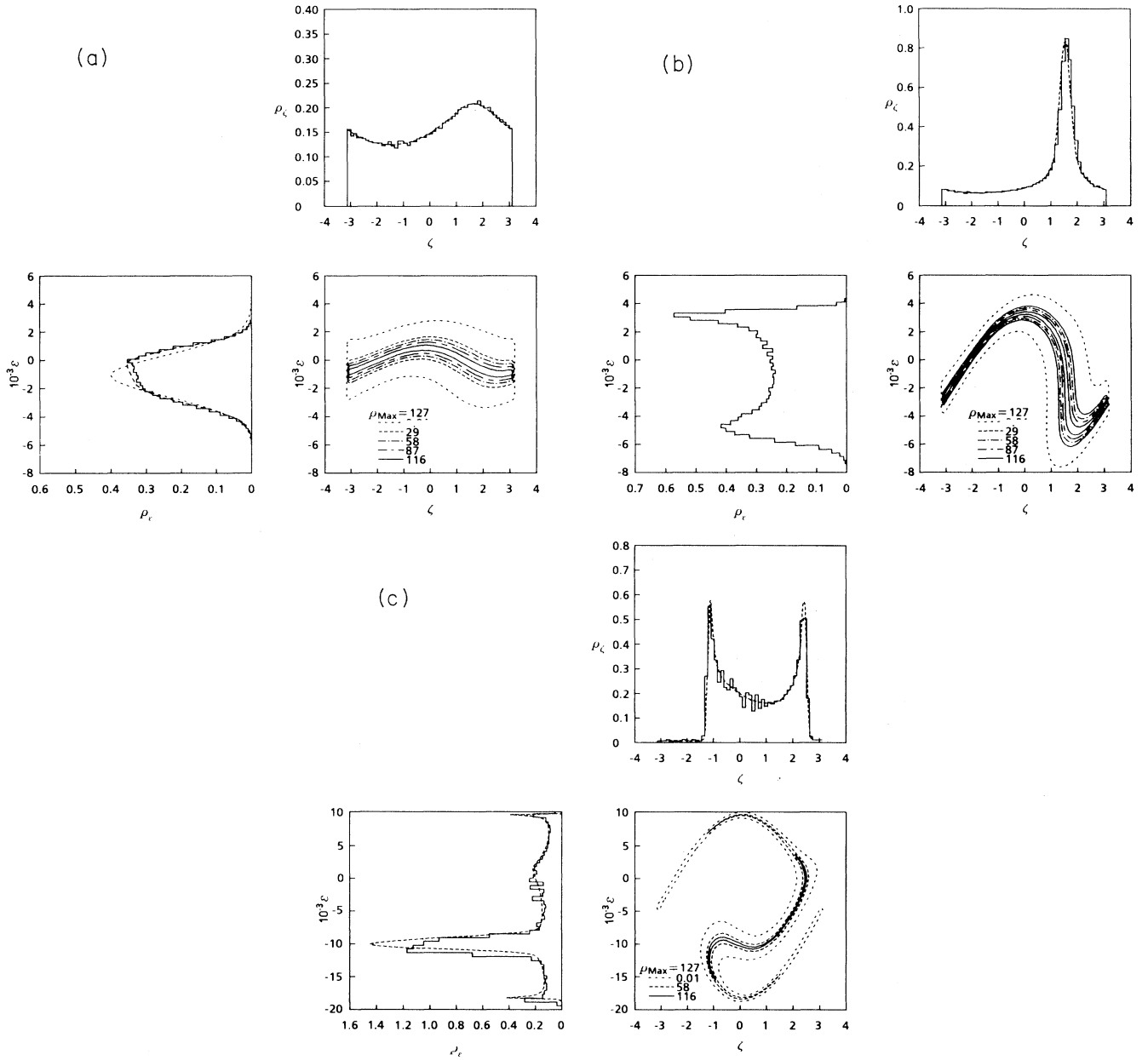
FIG. 1 (a) Integration of the FEL Liouville equation \rho_r, \rho_\zeta and phase-space distribution contour plots at \tau=1 . The histogram refers to the results of the simulation code. Parameters: N=40 , \sigma_\zeta(0)=5 \times 10^{-4} , \mu_\zeta(0)=4N\sigma_\zeta(0) , \xi=0.624 . (b) Same as (a), \xi=2.79 . (c) same as (a), \xi=12.48 .
